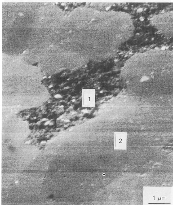
Figure 5 SEM micrographs of Al-12Si-1Mg/Si composite: (1) aluminium network, (2) silicon network.
