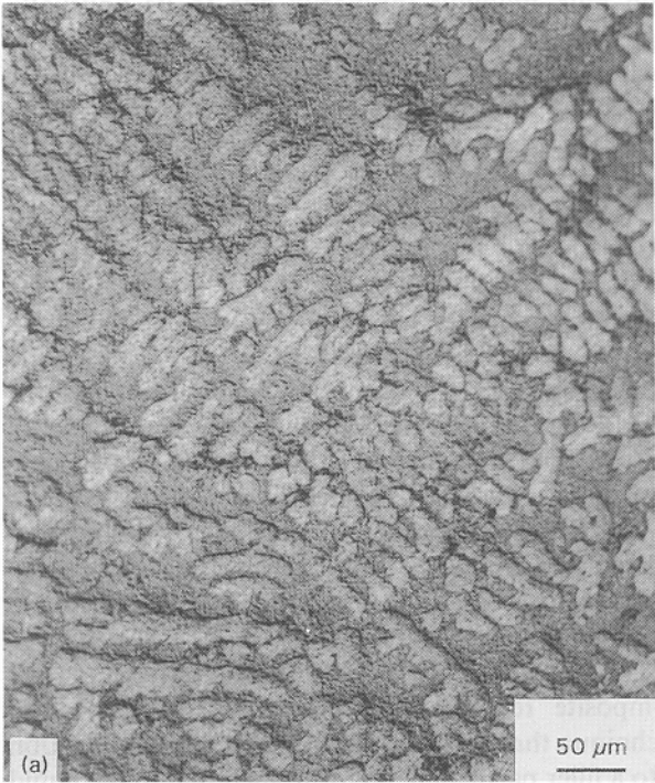
Figure 1 Optical micrographs of Al-Si-Mg alloys: (a) Al-12Si-1Mg, (b) Al-30Si-1Mg.
